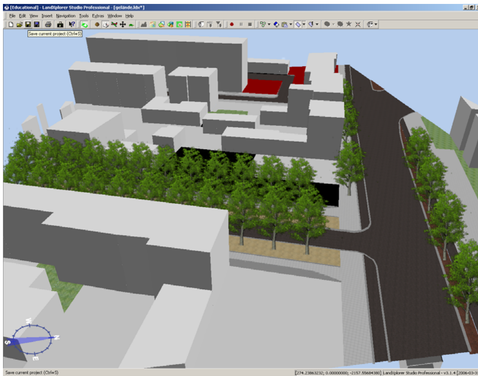
Figure 4: ST model from the example dataset Doringen
